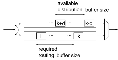
Fig. 10. Required size of routing FIFO buffers in order to ensure deadlock free operation.
