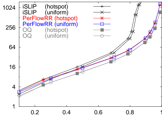
Fig. 13. Delay of non-hotspot destinations in the presence of hotspot/4 traffic; horizontal axis is the load to non-hotspot outputs; other parameters as in fig. 11.
