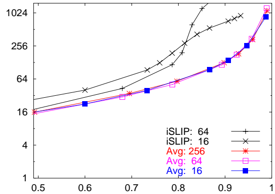
Fig. 14. Performance for various fabric sizes, 16 \times 16 to 256 \times 256 : average delay versus load, under bursty traffic in the presence of hot spots. The results are for the PerFlowRR cell distribution method.
