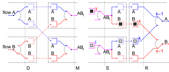
Fig. 5. Deadlock situation when flow merging precedes cell distribution. The participating switching elements are shown with dashed lines and the participating flows are indicated with A, B and AB. The numbers by the FIFO buffers denote the sequence number of the cell at the head of the buffer.
