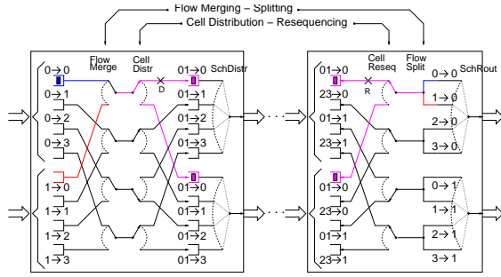
Fig. 4. Logical buffer organization of a distribution and the corresponding routing switching element.
