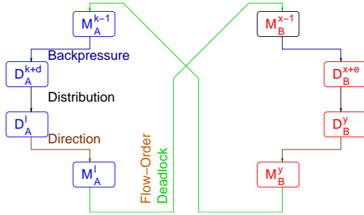
Fig. 9. The time-order graph. The nodes of the graph represent events of the form L_f^s and the arcs represent ordering relations between the events. The direction of an arc is from the older to the newer event.
