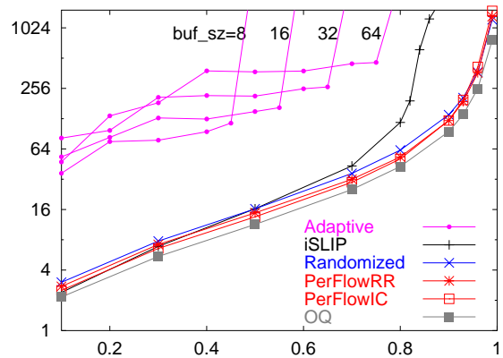
Fig. 12. Delay versus load for bursty/12 arrivals and uniform destinations; 64 \times 64 fabric made of 4 \times 4 elements; adaptive routing, randomized, 2-SLIP and ideal output queueing (OO) also shown for comparison.
