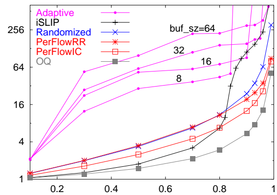
Fig. 11. Delay versus load for Bernoulli arrivals and uniform destinations; 64 \times 64 fabric made of 4 \times 4 elements; adaptive routing, randomized, 2-SLIP and ideal output queueing (OO) also shown for comparison.
