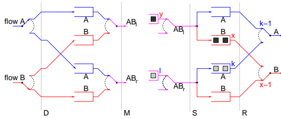
Fig. 6. Simplified but equivalent view of the deadlock situation shown in fig. 5.
