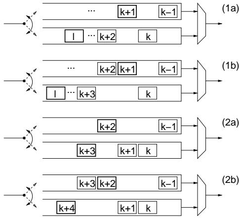
Fig. 8. Active cells allowed by cell distribution methods with maximum per-flow imbalance of 1.
