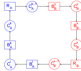
Fig. 7. The resource allocation graph for the deadlock situation. Circles represent cells, while rectangles represent resources which can be either buffer slots or resequencers.
